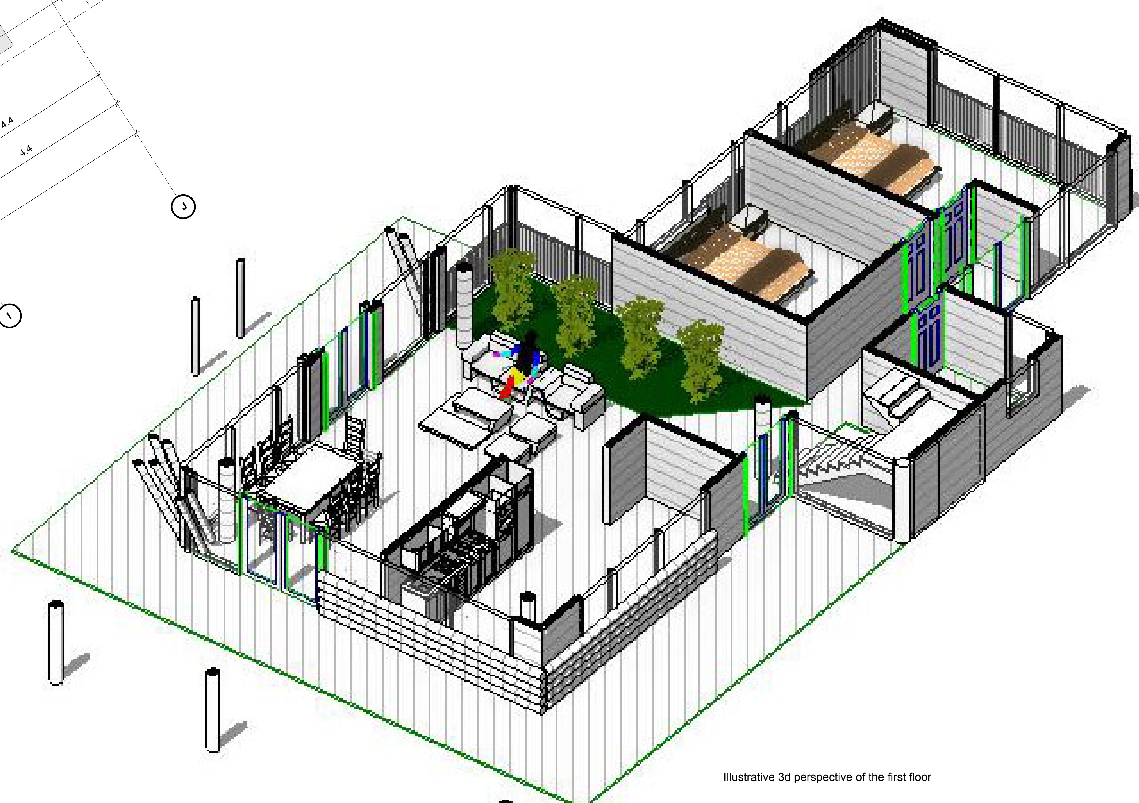
Illustrative 3d perspective of the first floor
