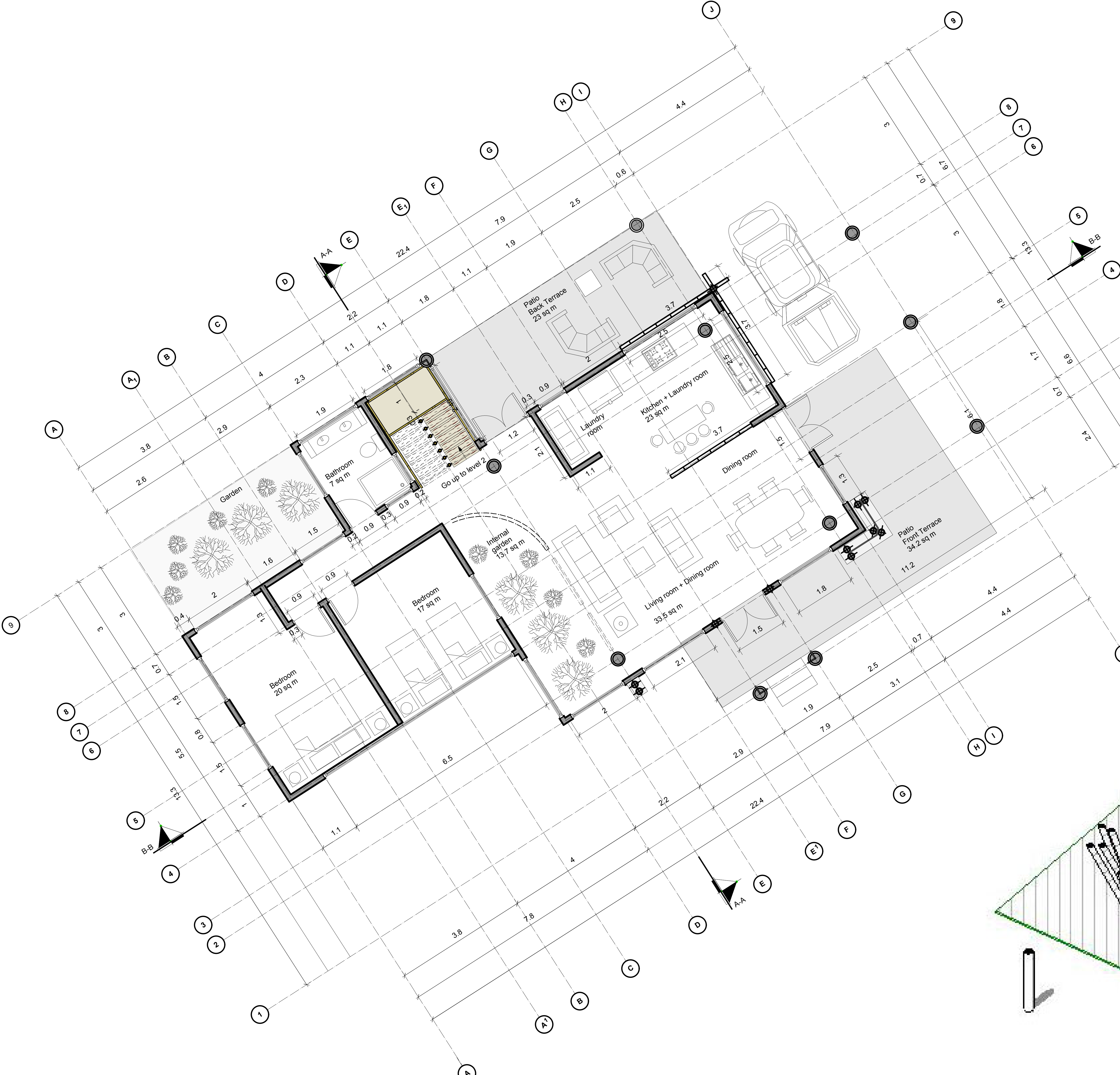
Architectural distribution plant First floor
